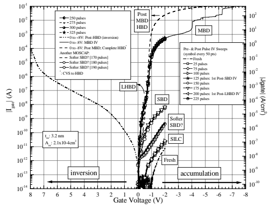
Figure 2: Similar to figure 1, but in addition, showing MBD and asymmetry of the I-V data with regards to inversion versus accumulation following HBD.
