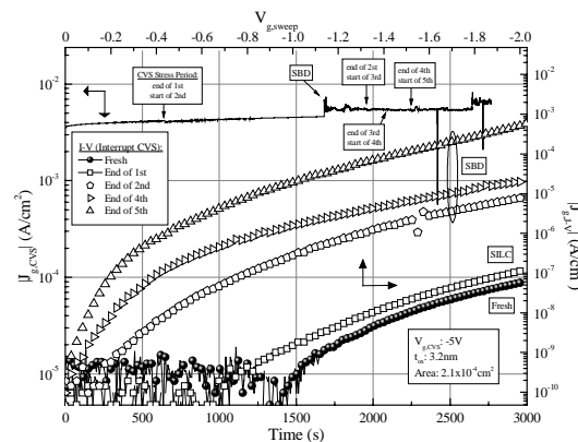
Figure 4: CVS J-t plot showing SBD and the intervals in which J-V measurements were performed. Corresponding J-V plots demonstrating SILC and SBD (symbol every 5 points).
