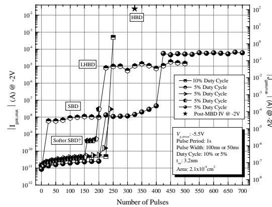
Figure 3: Current at -2V versus number of pulses at 5 and 10% duty cycles. Evident is SILC, soft SBD, SBD and LHBD. HBD after MBD is shown for comparison.
