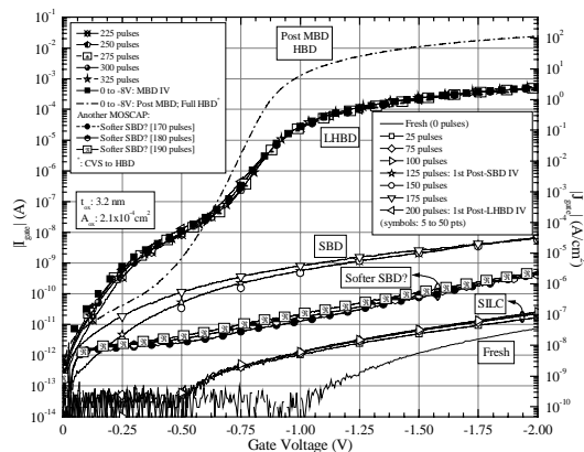
Figure 1: Pre- and post-PVS I-V data showing SILC, possible softer SBD, SBD, LHBD and complete HBD.
